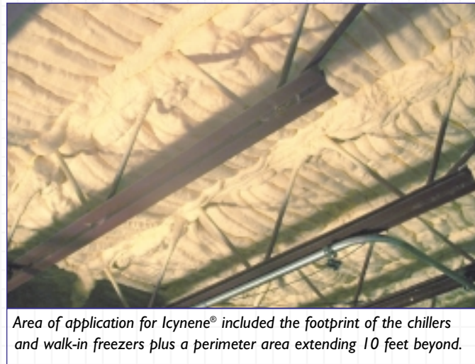
Icynene® insulation applied directly to the metal ceiling area below the chillers and walk-in freezers.
