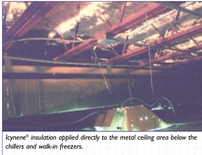
Area of application for Icynene® included the footprint of the chillers and walk-in freezers plus a perimeter area extending 10 feet beyond.
